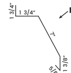
⑲ 29 Ga. Formed Valley TLFV19 10'2"
