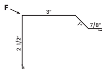
⑱ 29 Ga. Residential Rake TLRR18 10'2", 12'6", 14'6", 16'6"
