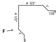
⑥ 29 Ga. "J" Channel TLJC6 10'2"
